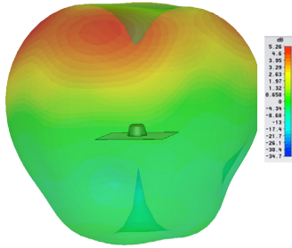
Typical 3D Pattern - Element 2 700MHz
