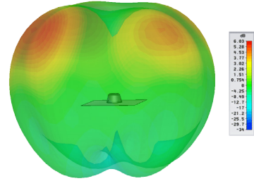
Typical 3D Pattern - Element 2 900MHz
