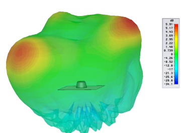
Typical 3D Pattern - Element 2 2600MHz
