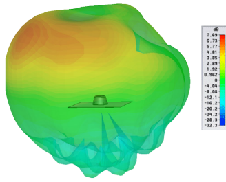
Typical 3D Pattern - Element 2 1800MHz
