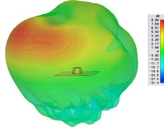
Typical 3D Pattern - Element 2 2000MHz
